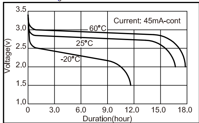
Discharge Characteristics
