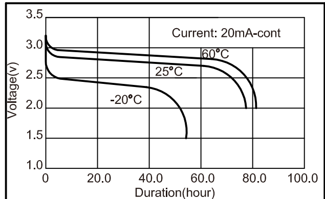
Discharge Characteristics
